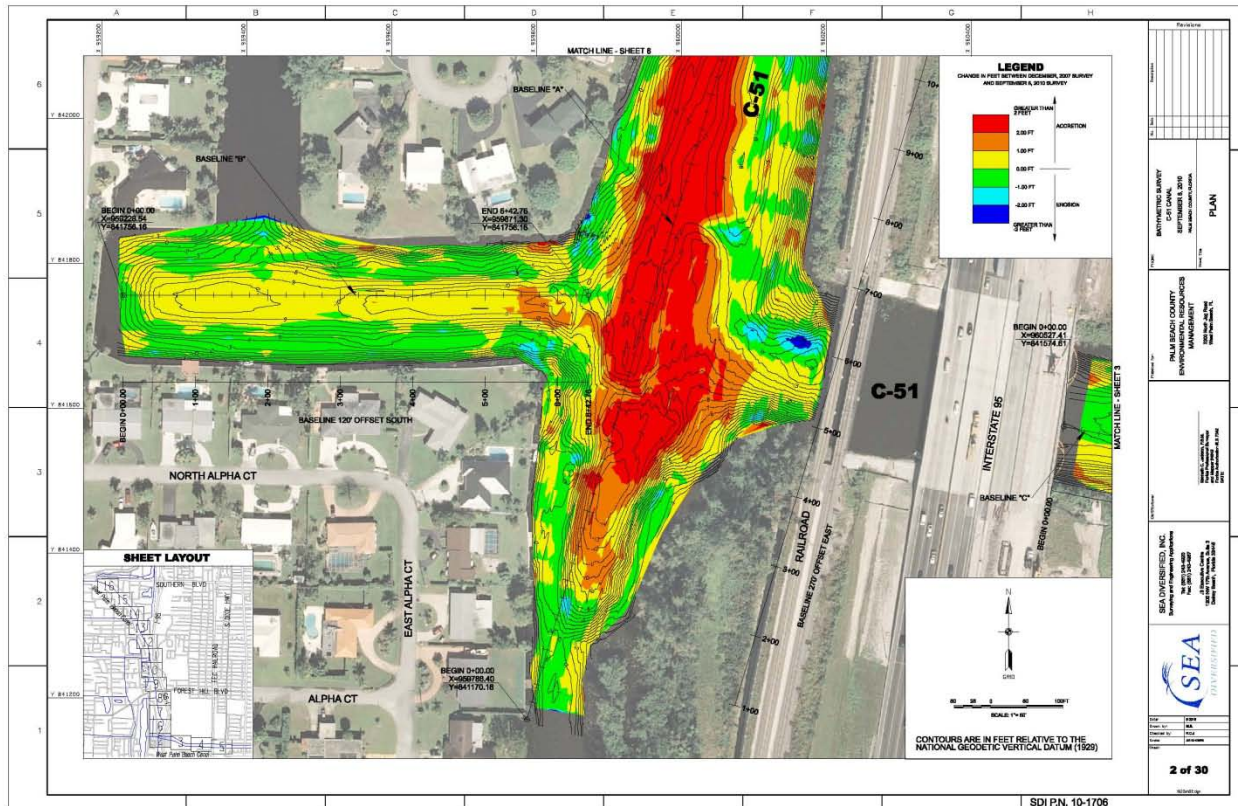
Figure 39. C-51 Sediment Trap Bathymetry, 2007-2010
