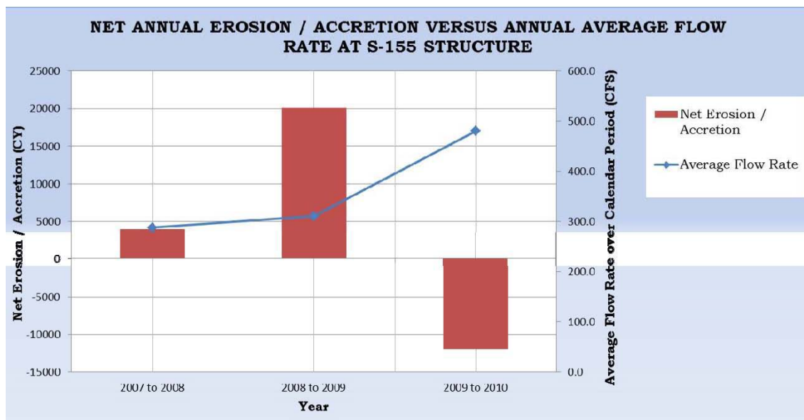
Figure 40. Net Annual Erosion/Accretion versus Annual Average Flow Rate at S-155 Structure
