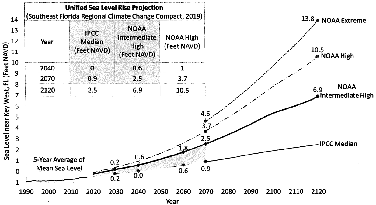
FIGURE 2: Unified Sea Level Rise Referenced to NAVD
