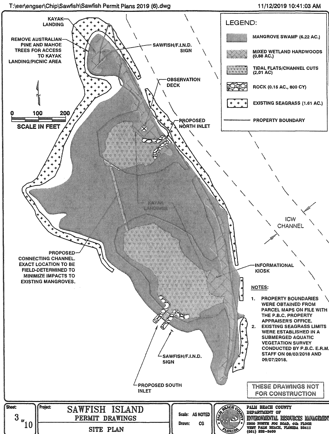
Figure 2: Site Plan
