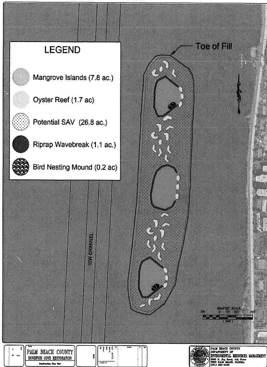
Figure 2 – Project Site Plan
