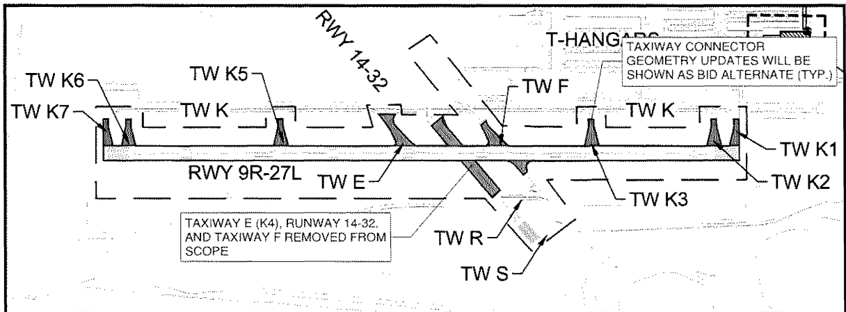
Figure 1 - Runway 9R-27L Construction Updated Scope
